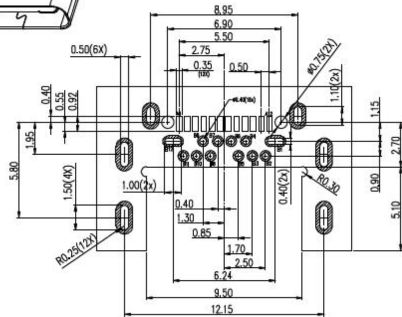
PCB LAYOUT (RECOMMENDED)
