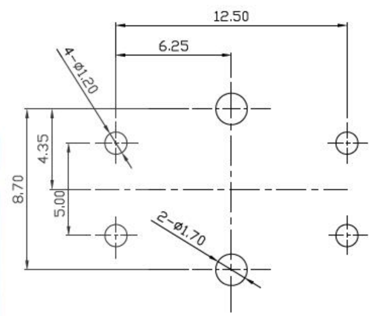
P.C.B MOUNTING PATTERN DIMENSION
