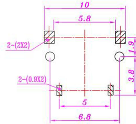
PCB LAYOUT
