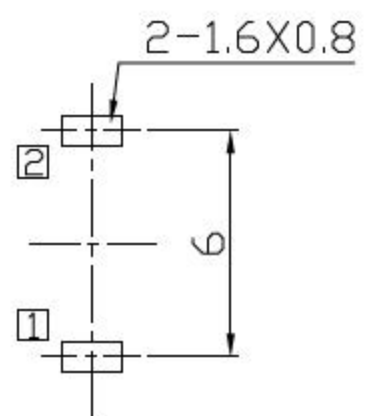
P.C.B Layout Tolerance: ±0.05mm (Copper-sided view)
