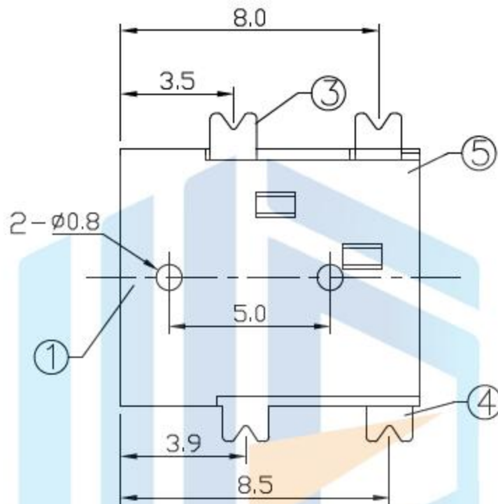
SCHMATIC
