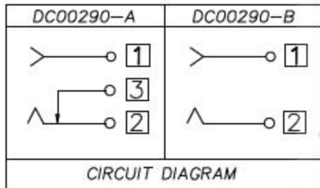
Circuit Diagram □: Terminal No.
