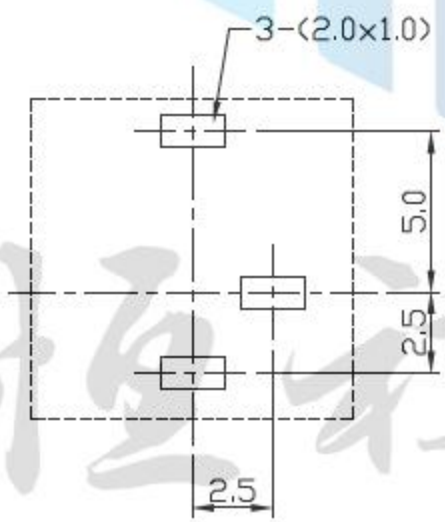
線路板開孔尺寸 P. C. B LAYOUT
