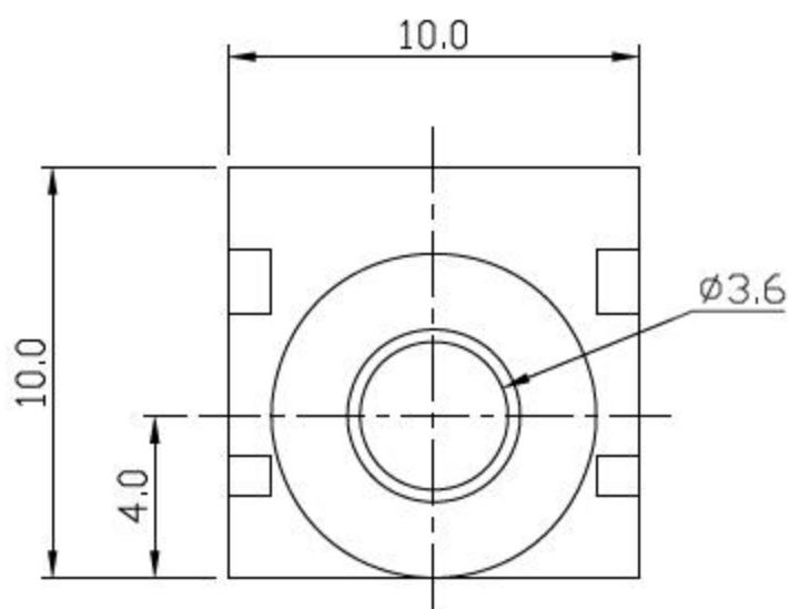
線路板開孔尺寸 P. C. B LAYOUT
