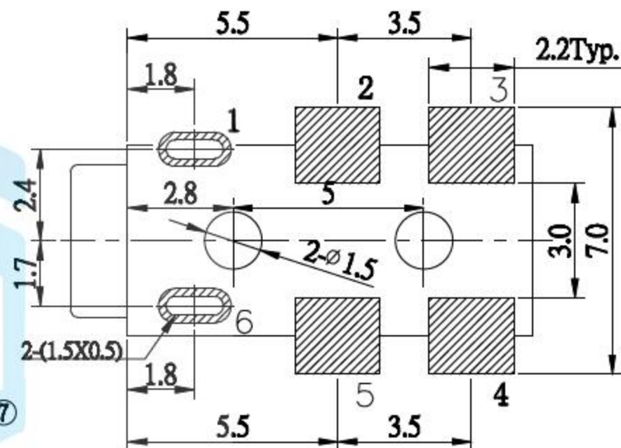
P.C.B LAYOUT MOUNTING PATTERN (TOP VIEW)
