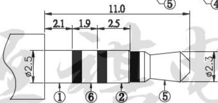
φ2.50mm 4 POLE PLUG
