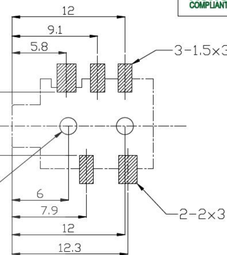
PCB LAYOUT
